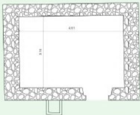
STONE GUEST HOUSE LIVING AREA : 14.30 m 2
