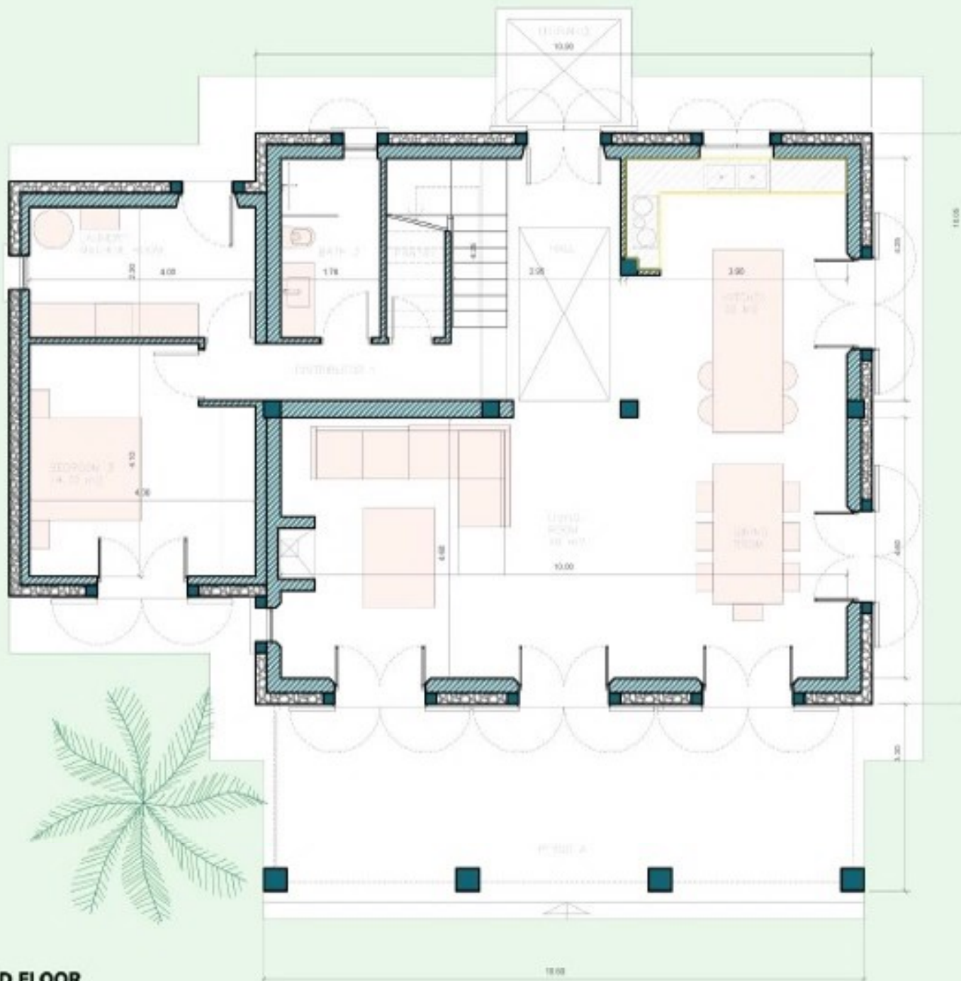
GROUND FLOOR BUILDING AREA : 141.50m 2 LIVING AREA : 118.30 m 2
