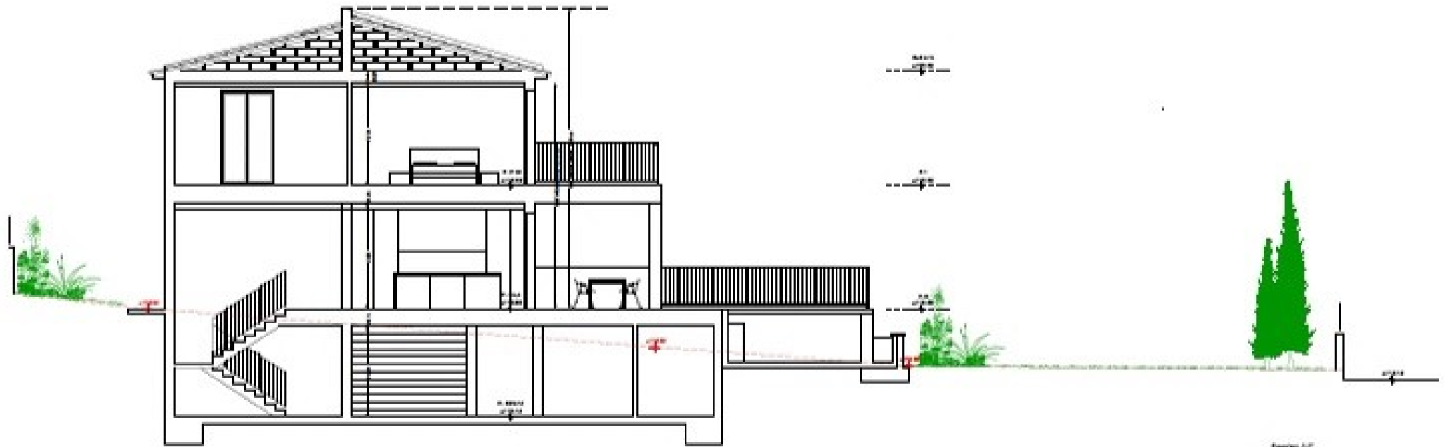
Section A-A 1/20
